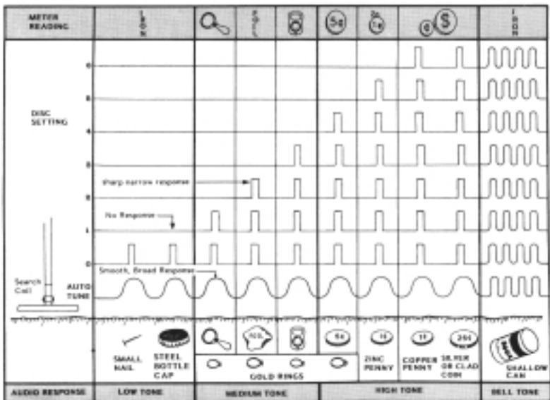
Figure 5. Typical 1280-X audio responses over 1 inch deep targets with search coil sweeping 1 to 2 inches above ground.
